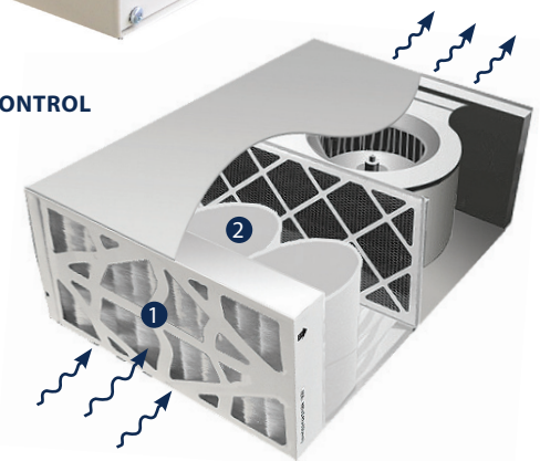
HOW AIR MOVES THROUGH TWO STAGE AIR FILTRATION SYSTEM
